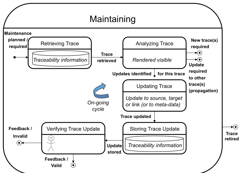
Fig. 6 Traceability maintenance
