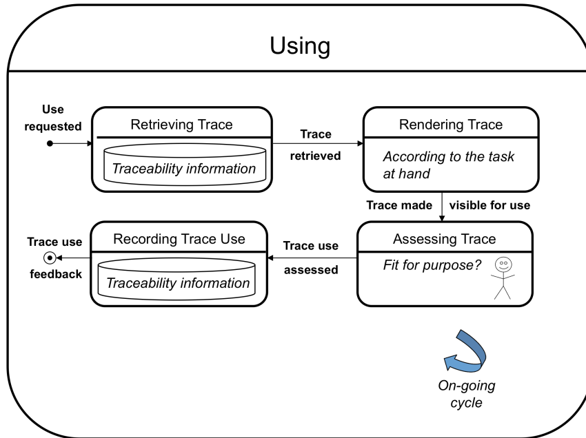
Fig. 7 Traceability use
