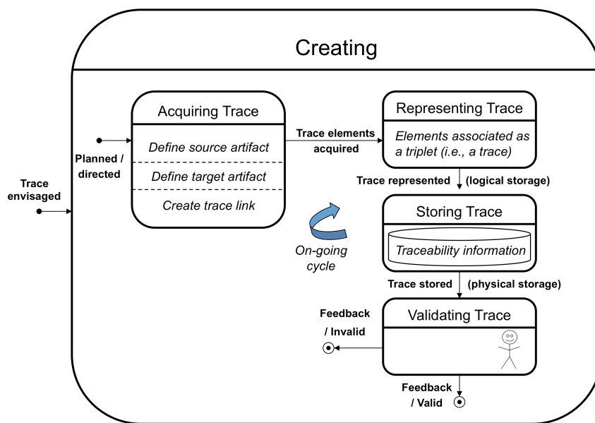
Fig. 5 Traceability creation
